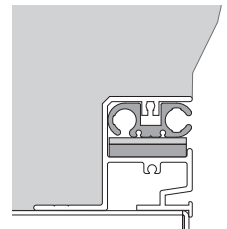
Track channel with vinyl retainer
