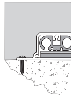
Deck-on-deck with Standard Track Channel
