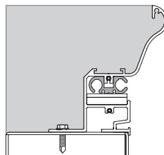
Vinyl-liner coping Standard
