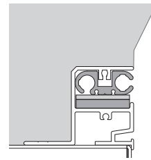
Track channel with vinyl retainer
