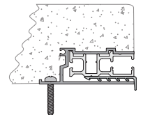
Undertrack with Dual-Race track channel
